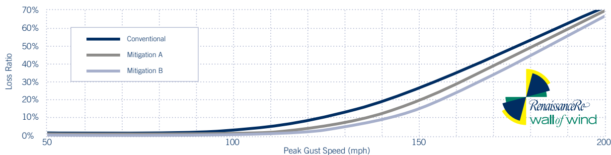
Projected vulnerability curves for mitigated and unmitigated roof surfaces.
